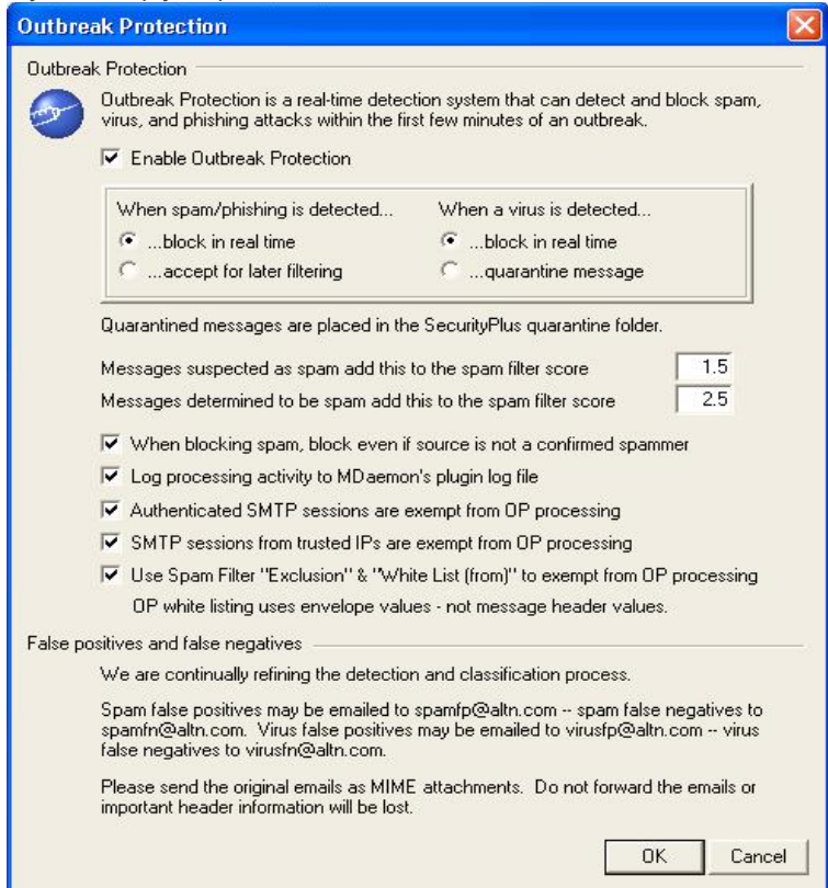
Configuration screen for Outbreak Protection (appears in MDAEMON's Security menu)
